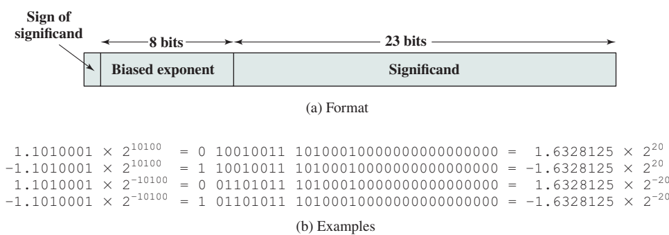
Figure 10.18 Typical 32-Bit Floating-Point Format
