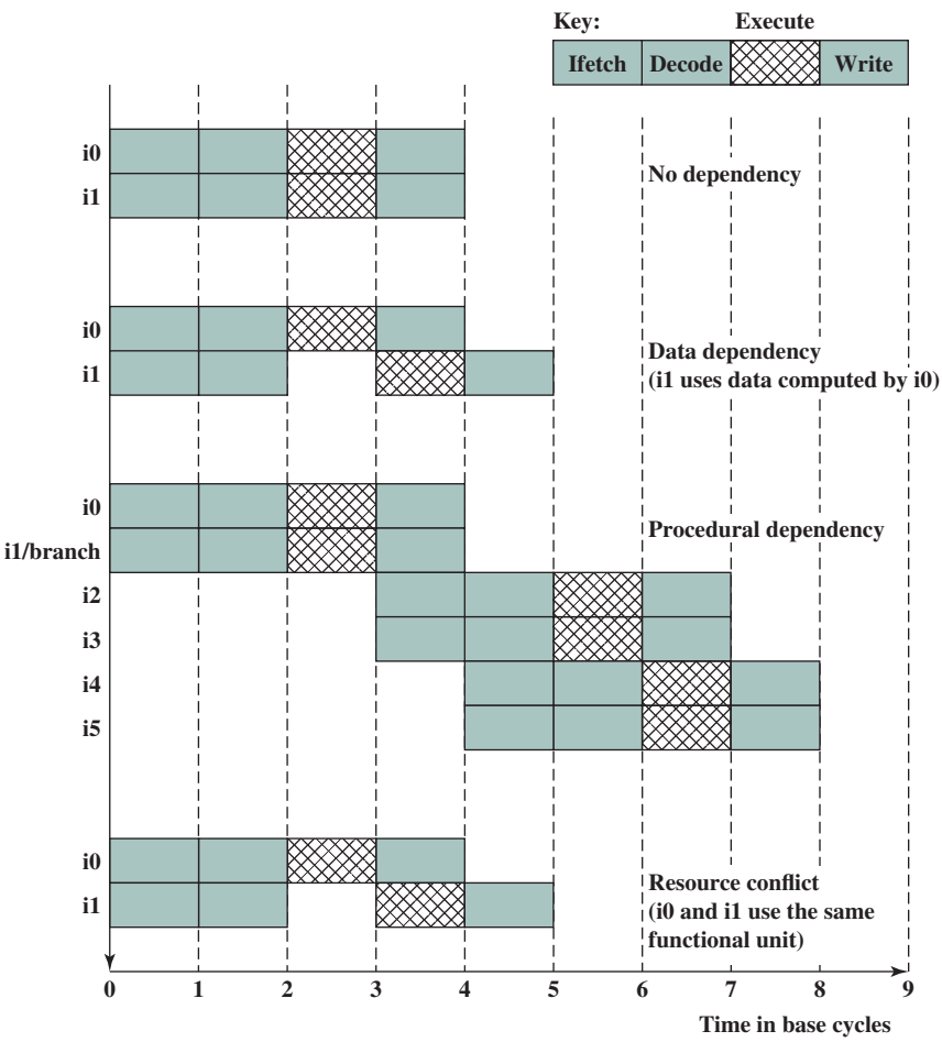
Figure 16.3 Effect of Dependencies
