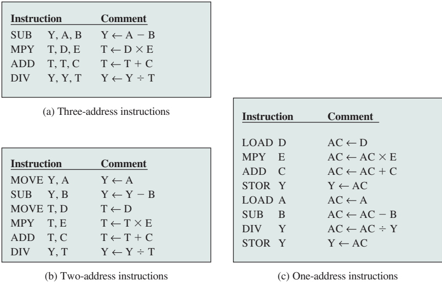
Figure 12.3 Programs to Execute Y = \frac{A - B}{C + (D \times E)}
