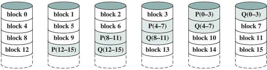
(g) RAID 6 (Dual redundancy)
