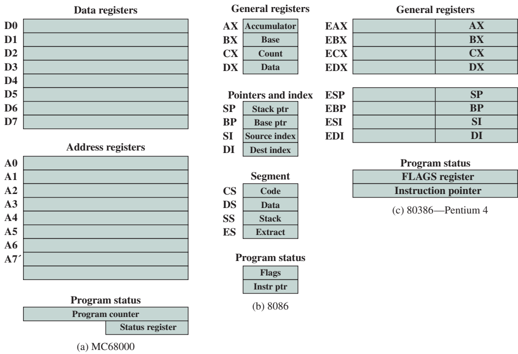
Figure 14.3 Example Microprocessor Register Organizations
