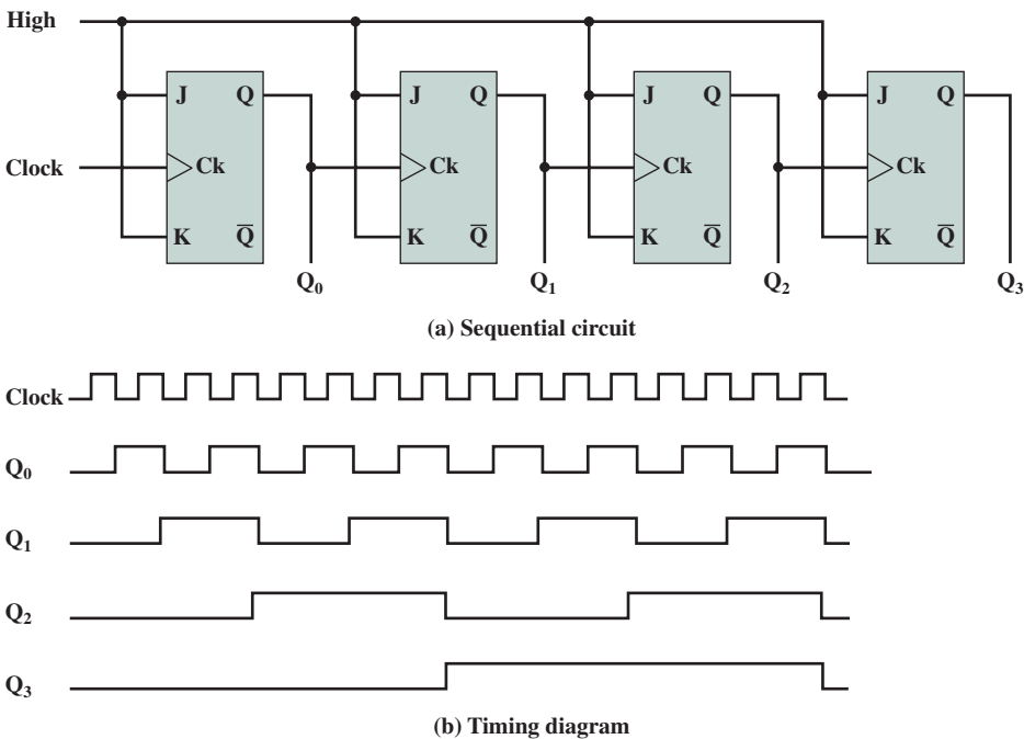
Figure 11.30 Ripple Counter
