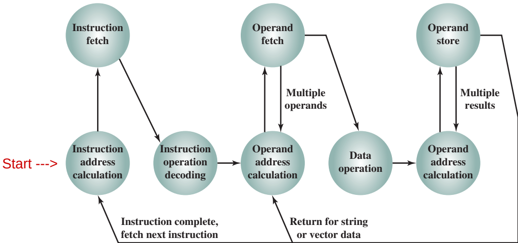
Figure 3.6 Instruction Cycle State Diagram
